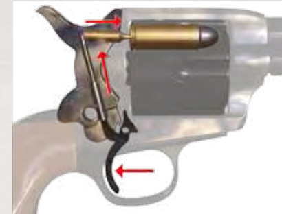
When the trigger is pulled from a fully-cocked position, the transfer bar engages the firing pin, locking it in the forward position until the trigger is released.
